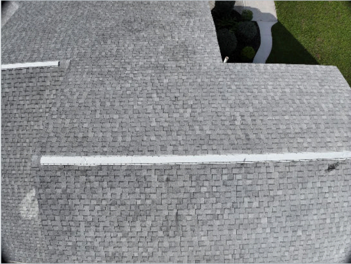
Photo 9: Ridge vent and adjacent slopes, dark marks below ridge
